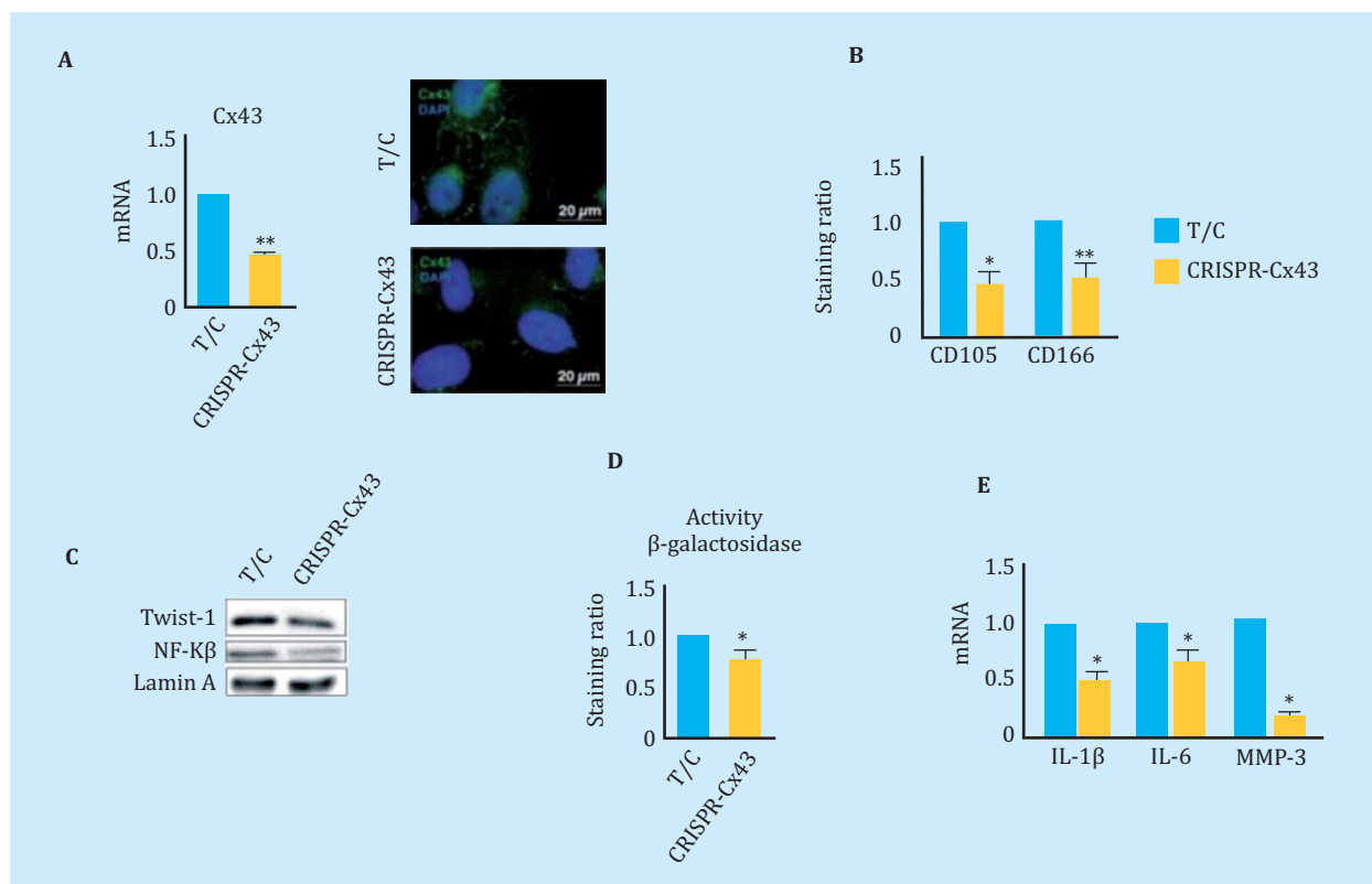
Figure 6. (A) On the left, gene expression levels of Cx43 in chondrocytes T/C-28a2 (T/C) and the same line with only one copy of Cx43 (CRISPR-Cx43). n=4, mean \pm SEM; * p <0.05; Mann-Whitney test. On the right, immunofluorescence for Cx43 (green) in chondrocytes T/C-28a2 (T/C) and the same line transfected with only one copy of Cx43 (CRISPR-Cx43). The nuclei have been stained with DAPI (blue). (B) Levels of the CD105 and CD166 markers measured by flow cytometry in the T/C-28a2 cell line with a single copy of Cx43 (CRISPR-Cx43) compared to the same line without transfection (T/C). n=7, mean \pm SEM; * p <0.05, ** p <0.01; Mann-Whitney test (C) Western blot to detect Twist-1, NF- \kappa B and N-Cadherin comparing a nuclear extract of the T/C-28a2 (T/C) line and from the same line with low amount of Cx43 (CRISPR-Cx43). Lamina protein A has been used as a load control. (D) Quantification by flow cytometry of \beta -galactosidase levels in the T/C-28a2 line (T/C) and the same line with only one copy of Cx43 (CRISPR-Cx43). n=4, mean \pm SEM; * p <0.05; Mann-Whitney test. (E) Gene expression levels of IL-1 \beta , IL-6 and MMP-3 measured in the same cells. n=4, mean \pm SEM; * p <0.05; Mann-Whitney test)
